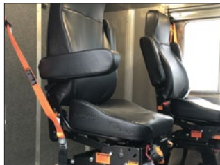
Full Size Passenger Seat
