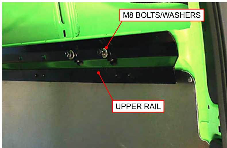
RH upper rail and fasteners
