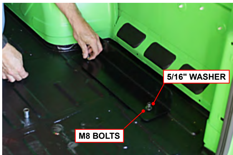
Floor mounting rail
