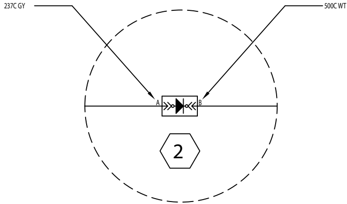
7.2 TO HEADLIGHT 282087-1
