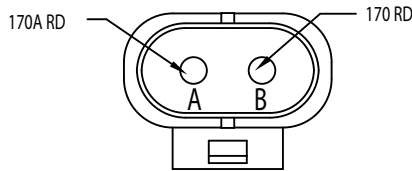
6.10 CLEARANCE LIGHT FUSE 12085030
