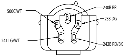
6.15 RIGHT LAMP FEED 12065158
