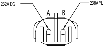
11.8 T/S FEED 12010973
