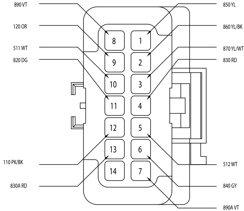
6.5 TO WIPER CONTROL MODULE 54201411
