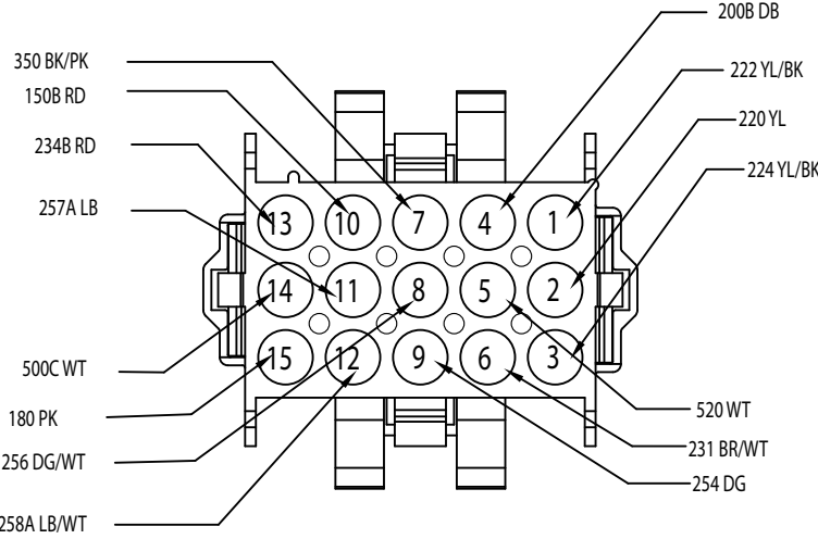
10.4 "A" PILLAR STANDARD TO 16400487 770030-1
