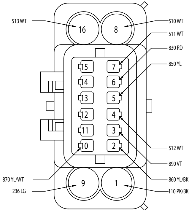
6.2 FORD CHASSIS CONNECTION-ENG-2 33486-1601
