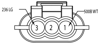
9.3/R RIGHT BACK-UP 282087-1
