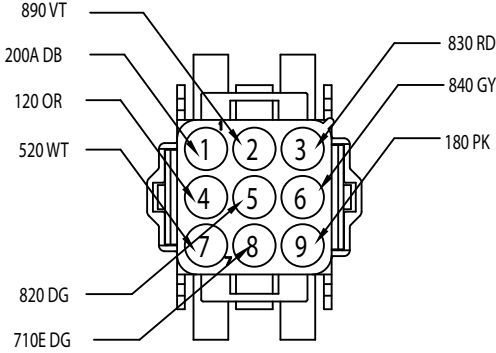
10.3 CHASSIS POWER FEED 770028-1
