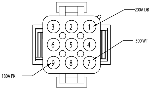
11.1 POWER FEED PLUG #1 770021-1
