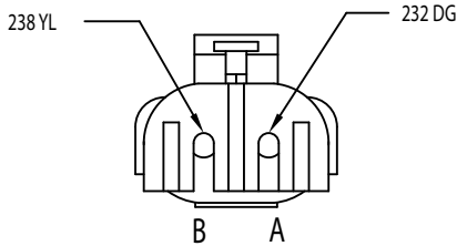
11.10 INTEGRATED TURN SIGNAL SOURCE 12015792
