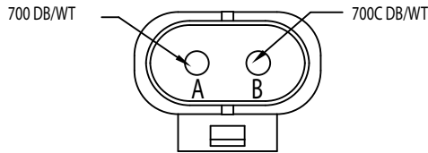
6.13 BLOWER MOTOR FUSE 12085030
