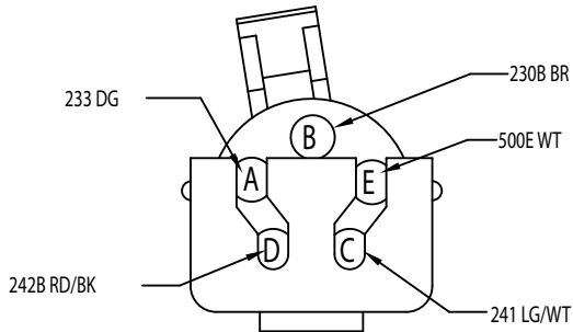
8.1/R RIGHT HEADLAMP DIST. 12034342
