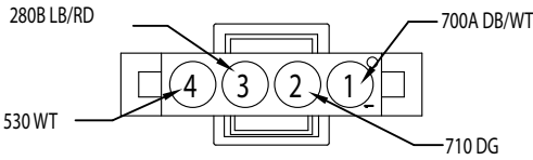
10.5 HVAC CONTROL TO SCS HARN 770019-1
