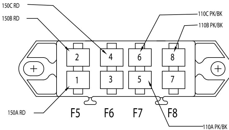
11.11 FUSE PANEL #1 (ETP) 12004943
