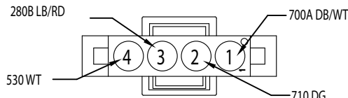
10.5 HVAC CONTROL TO SCS HARNESS 770019-1
