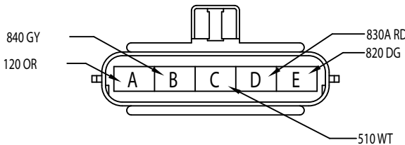
6.14 WIPER MOTOR 12084891
