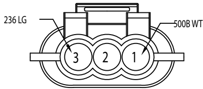
9.3/L LEFT BACK-UP 282087-1
