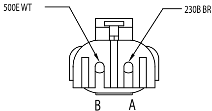
8.9/R RIGHT SIDE MARKER LIGHT 12015792
