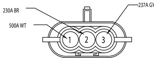
7.1 TO HEADLIGHT HARNESS 282105-1
