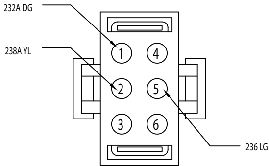
11.3 INTERIOR ROUTED WIRING 770020-1
