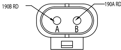
6.11 KEYLESS POWER FUSE 12085030
