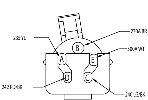
8.1/L LEFT HEADLAMP DIST. 12034342
