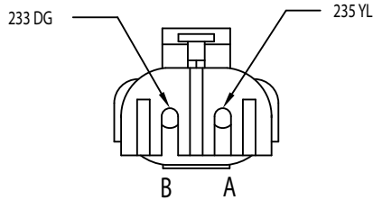
11.9 SPLIT TURN SIGNAL SOURCE 12015792
