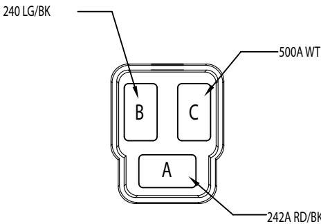
8.6/L LEFT HEADLIGHT 12077384
