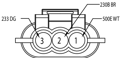
8.8/R RIGHT TURN/MARKER LIGHT 282087-1
