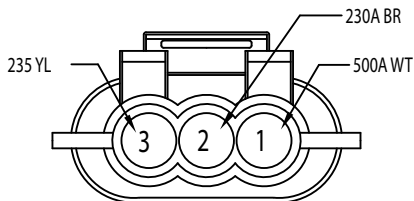
8.8/L LEFT TURN/MARKER LIGHT 282087-1
