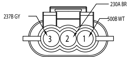
7.3 TO HEADLIGHT 282087-1
