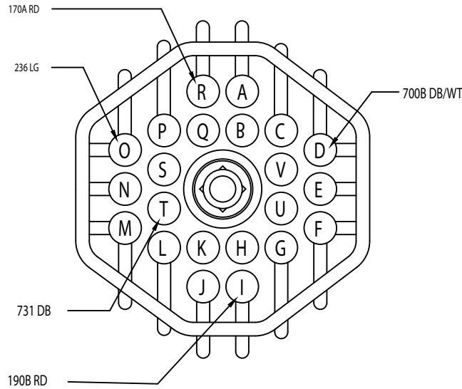
6.4 TO COWL CONNECTOR 15492521
