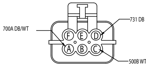
6.7 HVAC WATER VALVE 12052848
