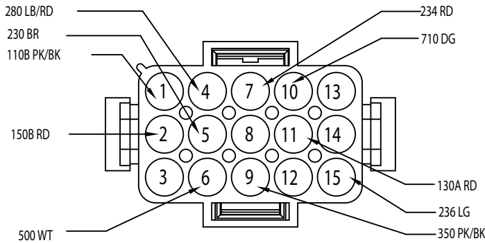
11.2 TO POWER FEED PLUG #2 770023-1
