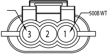
9.3/R RIGHT BACK-UP 282087-1
