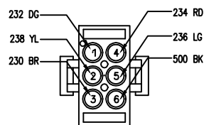
C418 INTERIOR ROUTED REAR LIGHTING 770020-1
