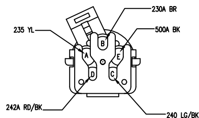
C205 LT HEADLAMP DIST 12034342
