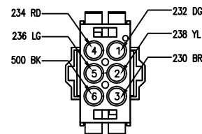
C419 INTERIOR ROUTED REAR LIGHTING 770027-1
