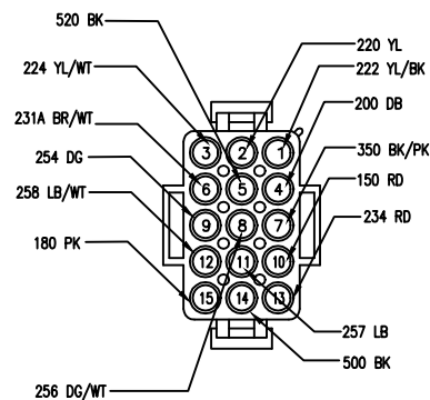
C412 "A" PILLAR(PILLAR) 770023-1
