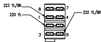
C300 REAR CARGO LIGHT SW 999-16716.001
