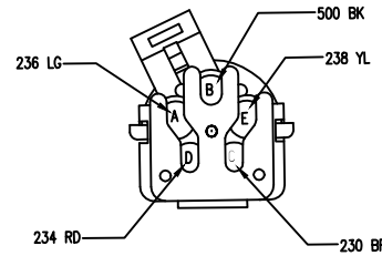
C631 LT REAR LAMP FEED 12034342
