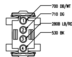
C331 HVAC CONN.(SCS) 770209-1
