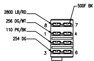
C302 AUXILIARY SW(IGNITION) 999-16716.001
