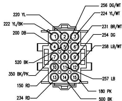
C410 "A" PILLAR(DASH) 770029-1
