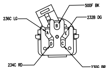
C633 RT REAR LAMP FEED 12034342
