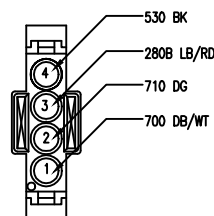
C330 HVAC CONN.(SCS) 770019-1
