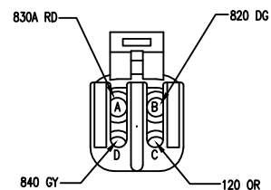
C207 WIPER MOTOR 12015798
