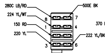
C301 AUXILIARY SW(BATTERY) 999-16716.001
