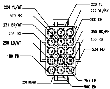
C411 "A" PILLAR(PILLAR) 770023-1
