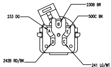
C203 RT HEADLAMP DIST 12034342
