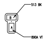
C206 WASHER PUMP 480115-1
