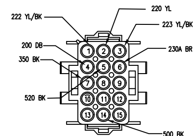
C413 "A" PILLAR(ROOF) 770029-1
