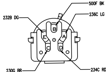
C634 RT REAR LAMP DIST 12065158
