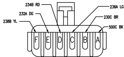
C610 REAR LAMP DIST 12015799
