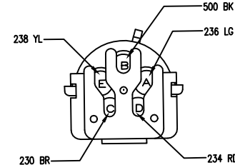
C632 LT REAR LAMP DIST 12065158
