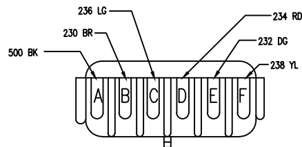
C609 REAR LAMP FEED 12010975
