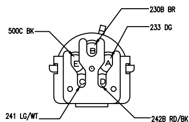
C202 RT HEADLAMP FEED 12065158
