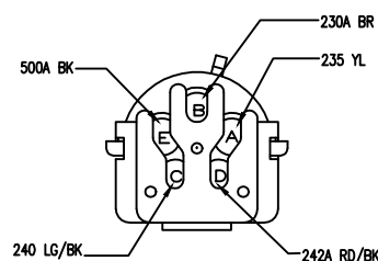
C204 LT HEADLAMP FEED 12065158
