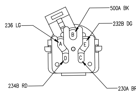
C634 RT REAR LAMP DIST 12065158
