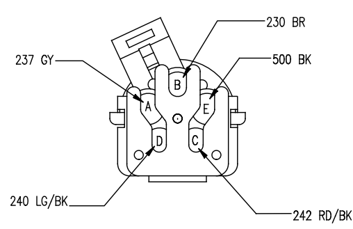
C205 LT HEADLAMP DIST 12034342
