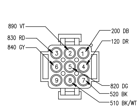
C110 POWER FEED #1 PLUG 770021-1
