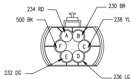
C117 FORD TAILLIGHT CONN 12010975
