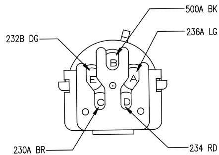
C633 LT REAR LAMP FEED 12034342
