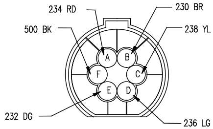
C611 REAR LAMP FEED 12015799
