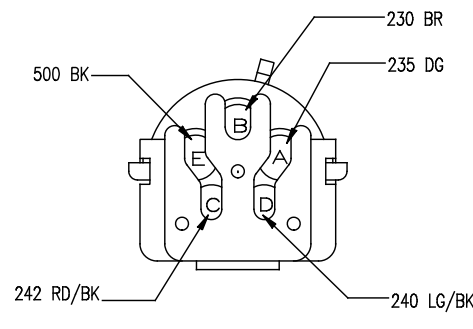
C202 RT HEADLAMP FEED 12034342
