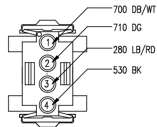
C331 HVAC CONN.(SCS) 770209-1
