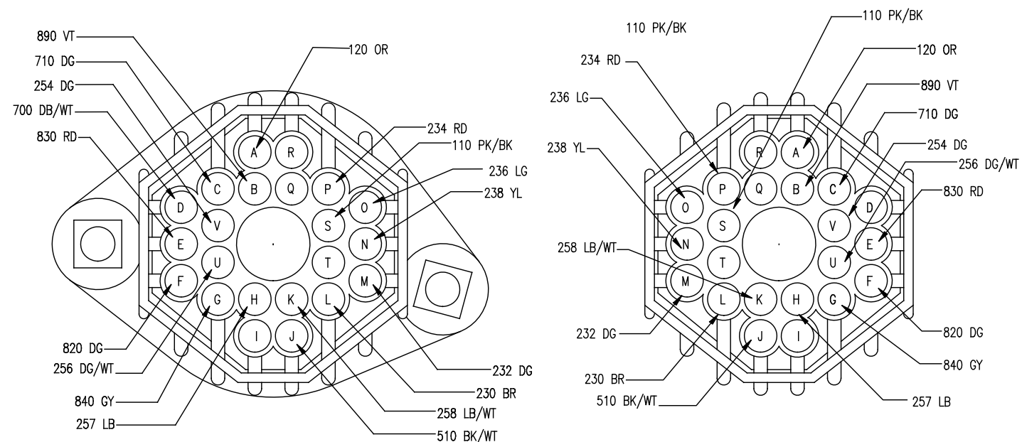
C100 COWL CONNECTOR 12020991
