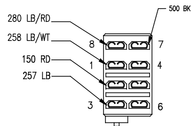
C303 AUXILIARY SW(BATTERY) 999-16716.001
