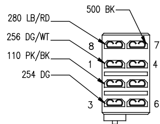
C302 AUXILIARY SW(IGNITION) 999-16716.001
