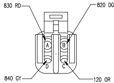
C207 WIPER MOTOR 12015798
