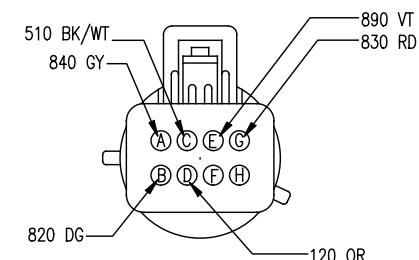
C110 POWER FEED #1 PLUG 770021-1
