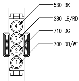
C330 HVAC CONN.(SCS) 770019-1
