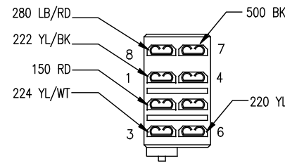
C301 AUXILIARY SW(BATTERY) 999-16716.001
