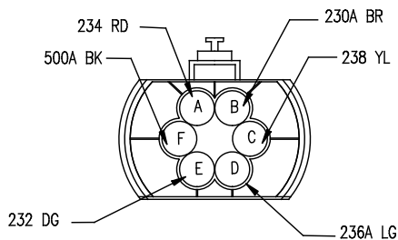
C610 REAR LAMP DIST 12010975
