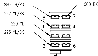
C300 REAR CARGO LIGHT SW 999-16716.001
