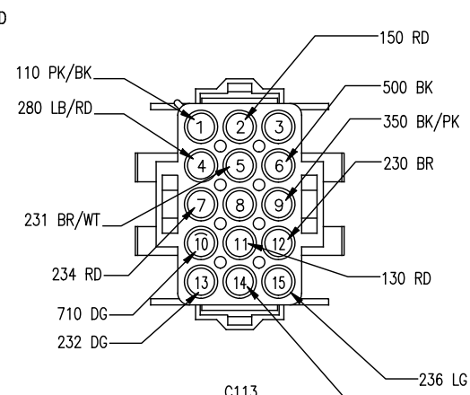
C113 POWER FEED #2 CAP 770030-1
