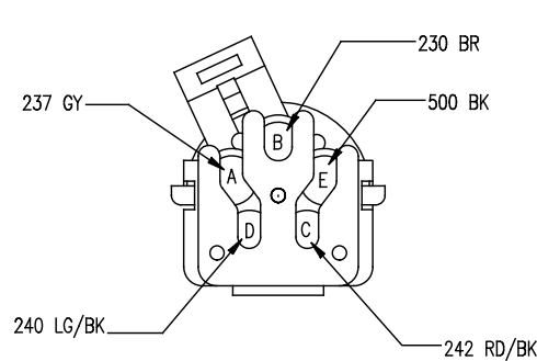
C203 RT HEADLAMP DIST 12065158
