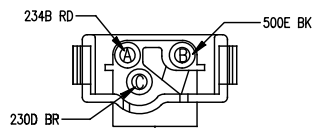
C636 RT STOP/TAIL MOLDED CONN.
