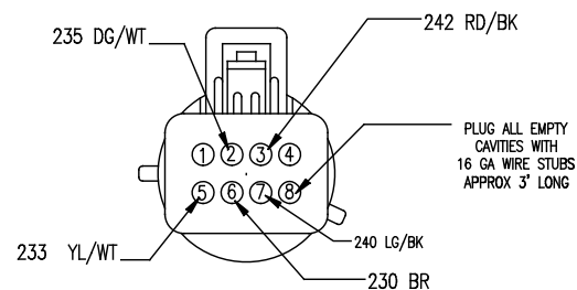
C200 HEAD LAMP CONN 12089040
