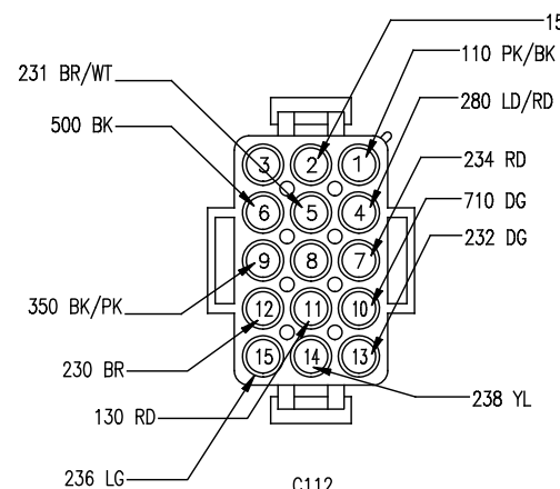
C112 POWER FEED #2 PLUG 770023-1
