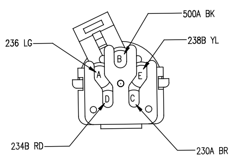
C632 RT REAR LAMP DIST 12065158
