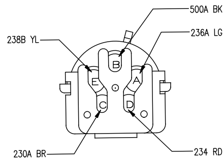
C631 RT REAR LAMP FEED 12034342
