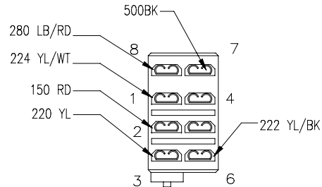
C301 AUXILIARY SW(BATTERY) 999-16716.001
