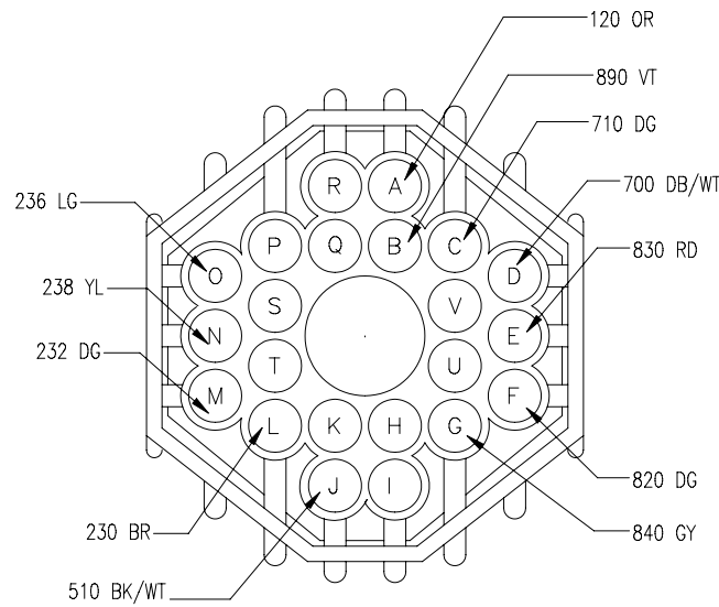
C101 COWL CONNECTOR 12020005
