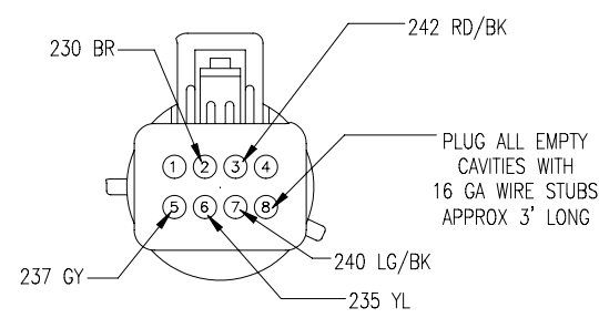
C200 HEADLAMP JUMPER CONNECTOR 12089040
