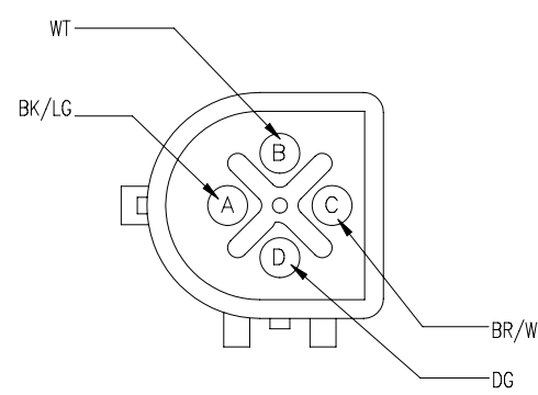
C118 FORD TAILLIGHT CONNECTOR F2US-14A411-D (BROWN CONNECTOR)
