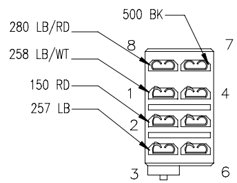
C303 AUXILIARY SW(BATTERY) 999-16716.001
