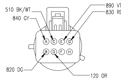
C115 INST-1 F2US-17B587-B
