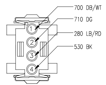
C331 HVAC CONN.(SCS) 770209-1
