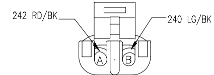
C210 DRL(DAYTIME RUNNING) 12015792
