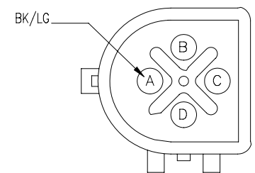
C117 FORD TAILLIGHT JUMPER F2US-14A411-B (ORANGE CONNECTOR)
