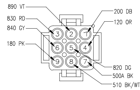
C110 POWER FEED #1 PLUG 770021-1
