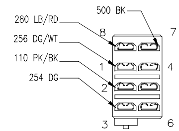
C302 AUXILIARY SW(IGNITION) 999-16716.001
