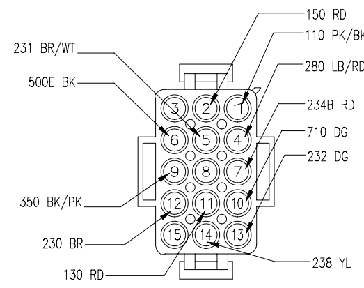
C112 POWER FEED #2 PLUG 770023-1 130 RD
