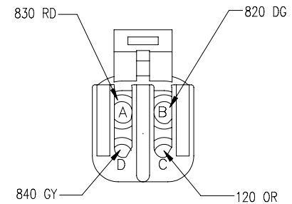
C207 WIPER MOTOR 12015798
