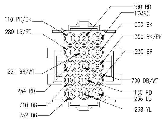
C113 POWER FEED #2 CAP 770030-1
