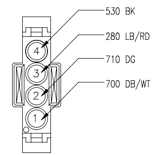
C330 HVAC CONN.(SCS) 770019-1
